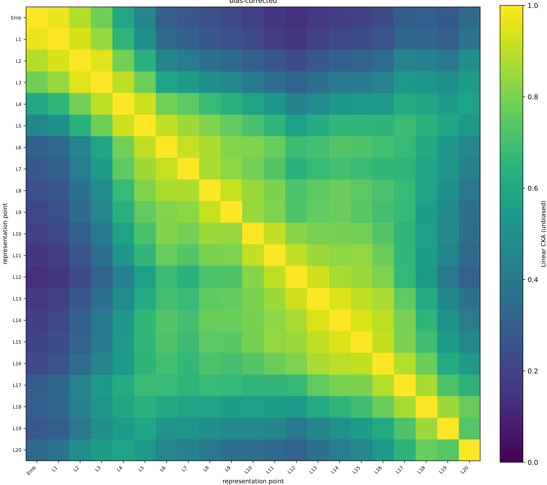
TimesFM-3 Uber TLC (PT-ID) — token 15 unbiased linear CKA | train split | N=1394 | independent-representation floor 0.000 bias-corrected
