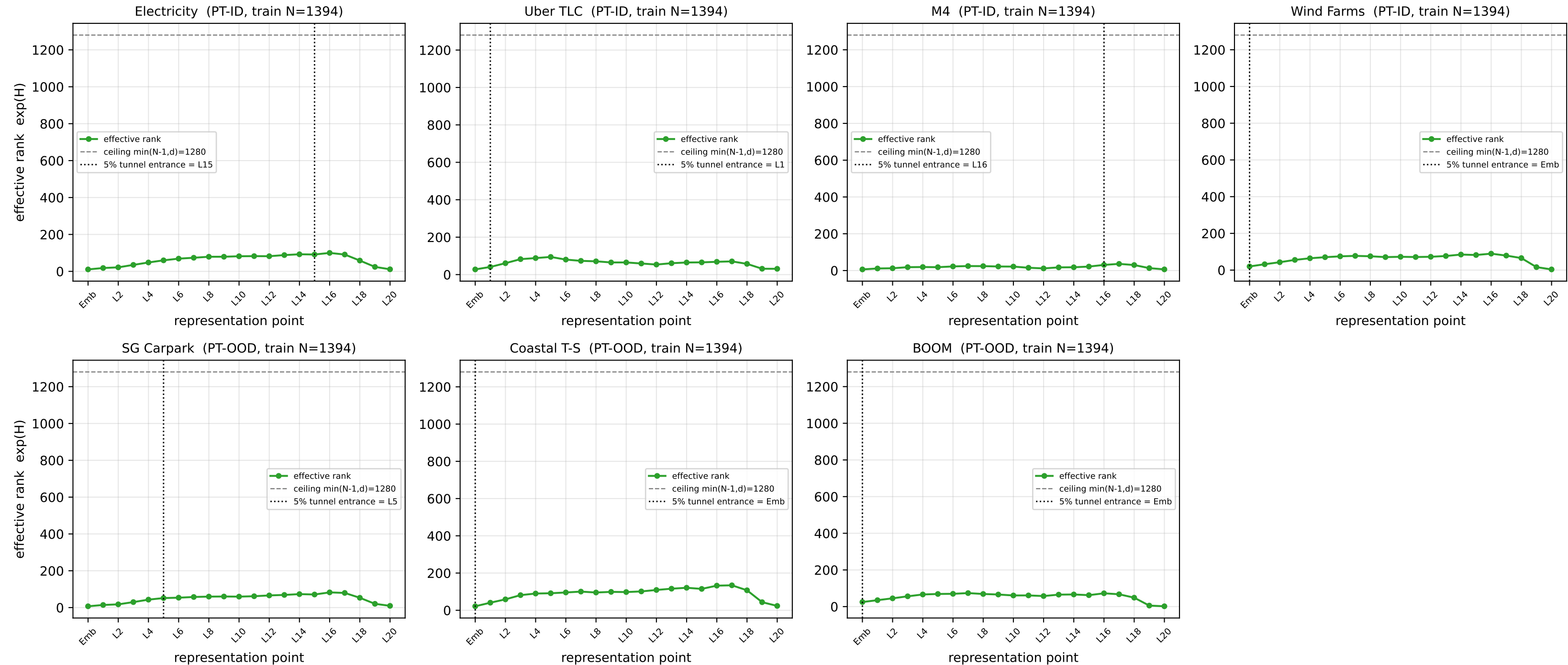
TimesFM-3 last-context-token ( h_{l,15} ) — effective rank \exp(H)
