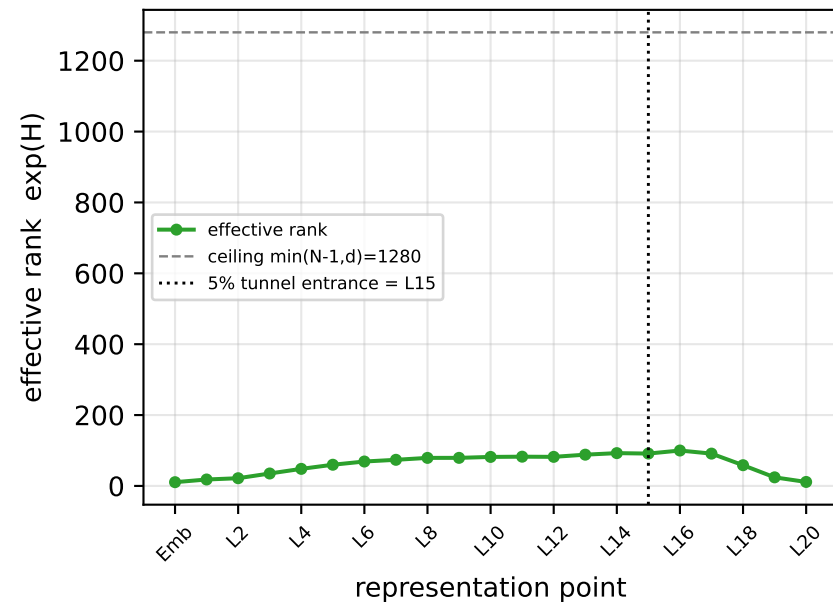
Electricity (PT-ID, train N=1394)
