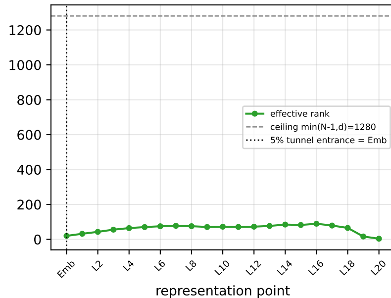
Wind Farms (PT-ID, train N=1394)
