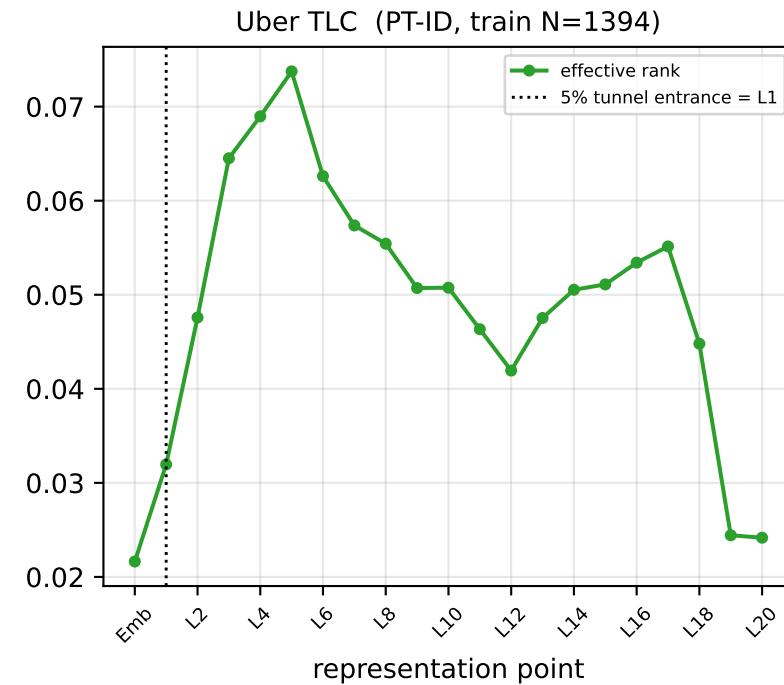
TimesFM-3 last-context-token ( h_{l,15} ) — effective rank / d ( d = 1280 )
