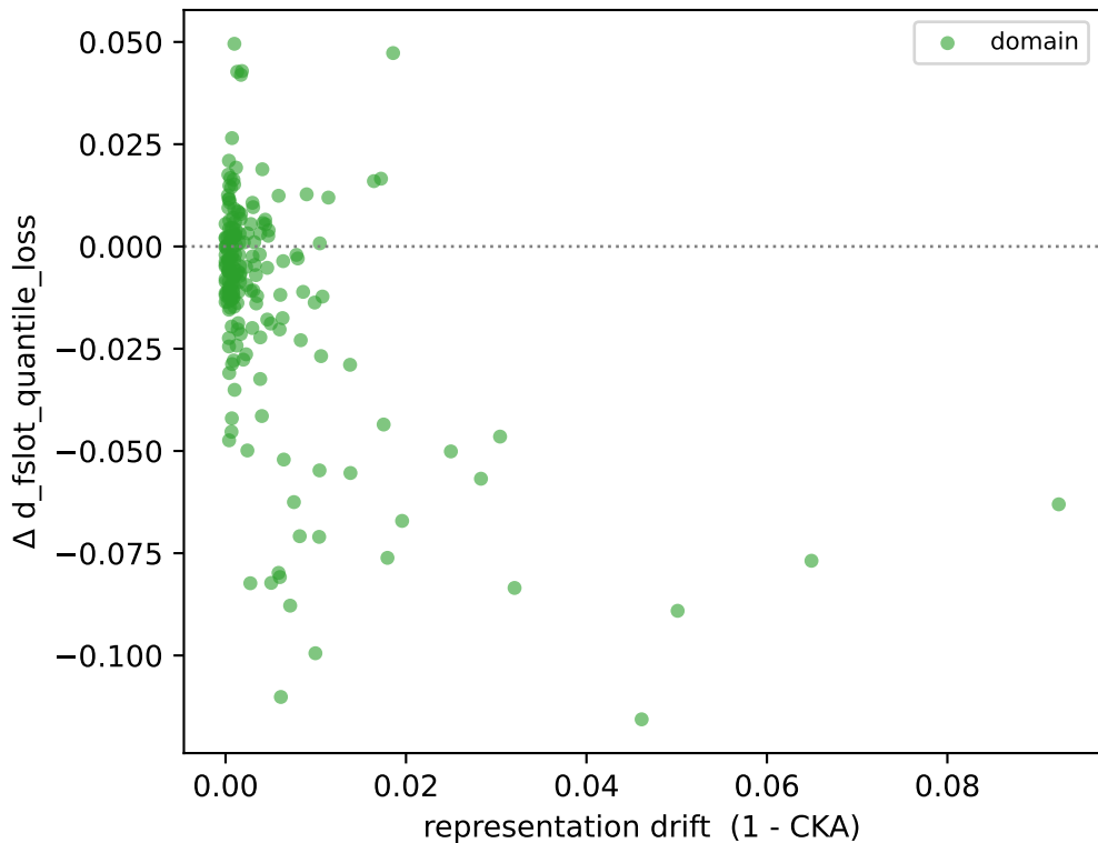
d_fslot_quantile_loss
