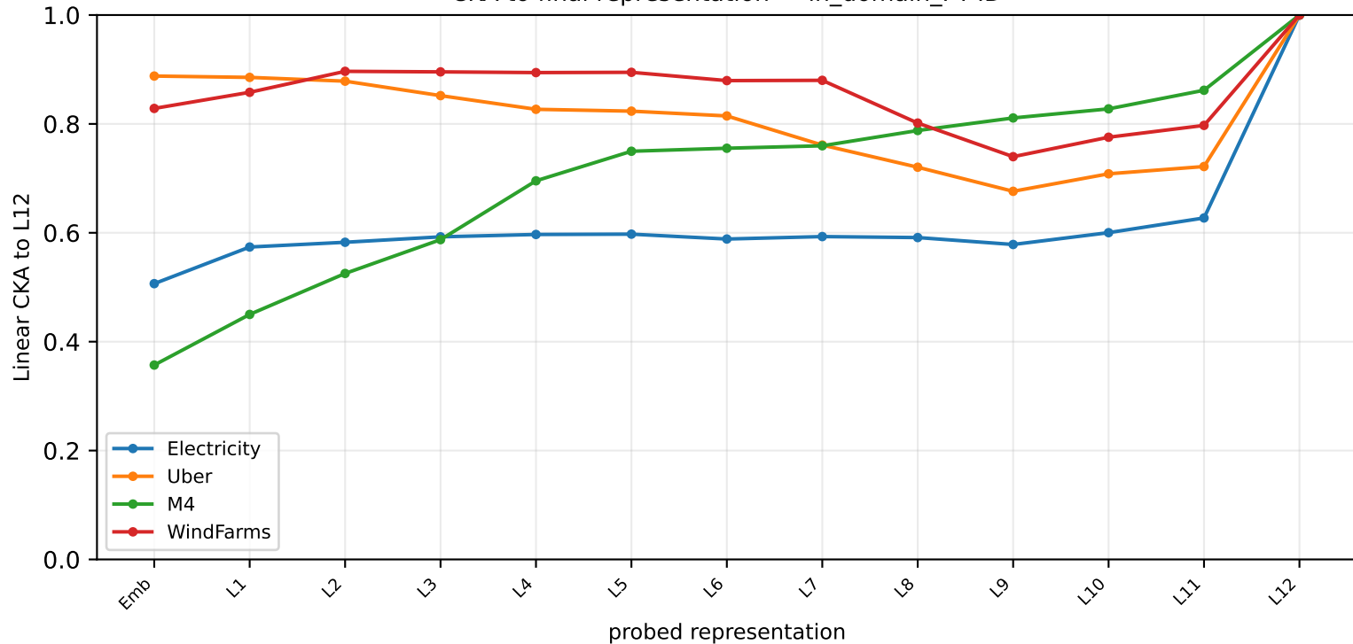
CKA to final representation — in_domain_PT-ID
