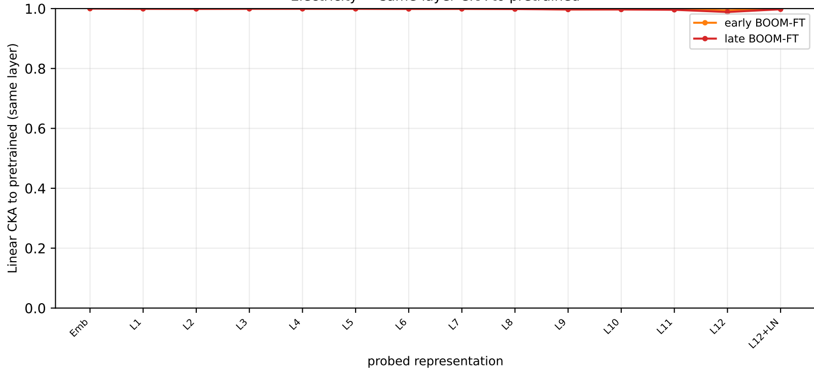
Electricity — same-layer CKA to pretrained
