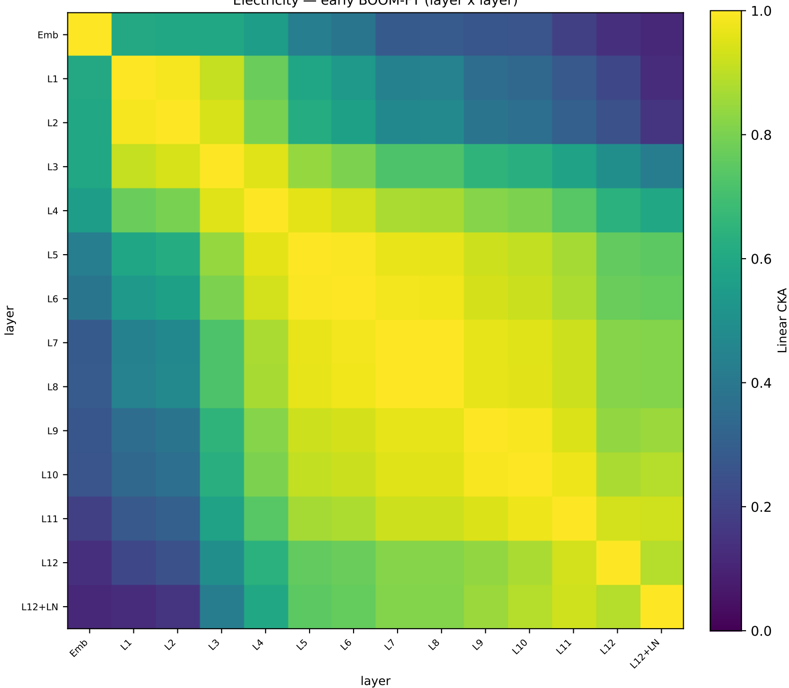
Electricity — early BOOM-FT (layer x layer)
