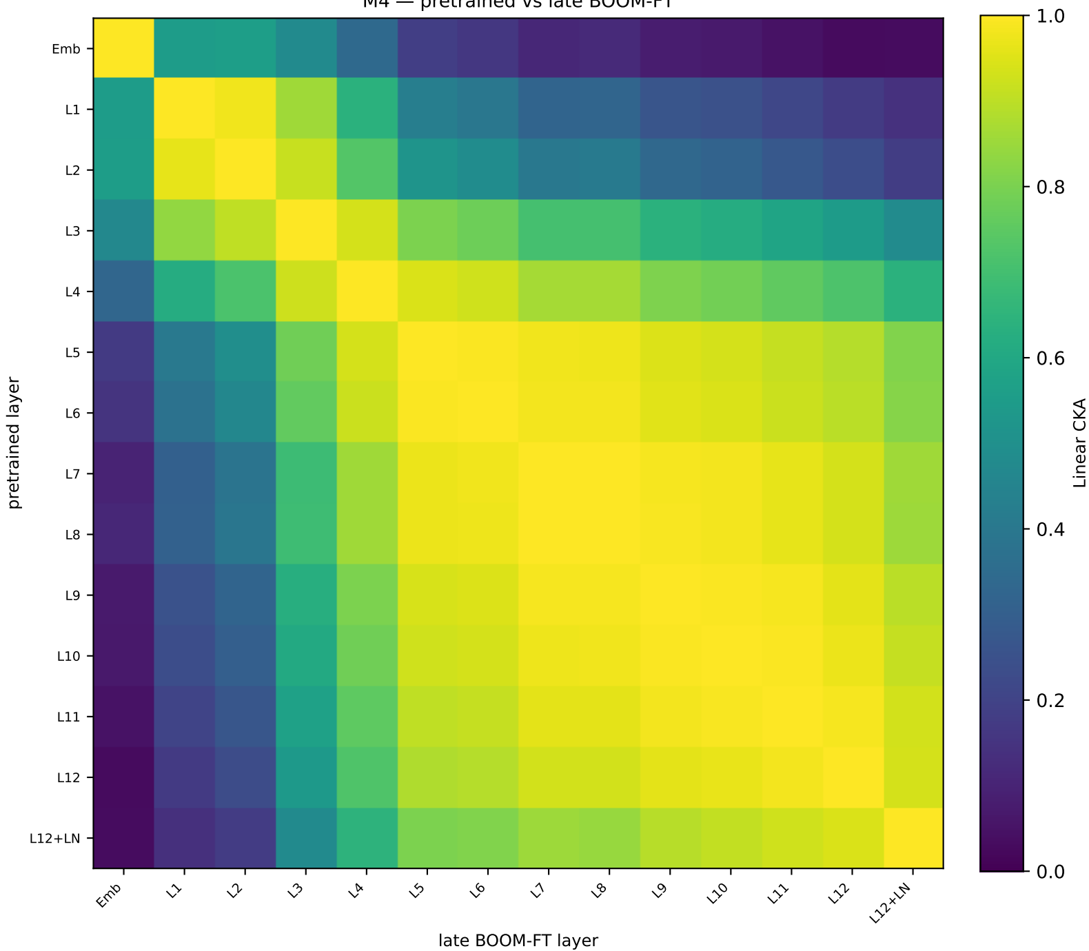
M4 — pretrained vs late BOOM-FT
