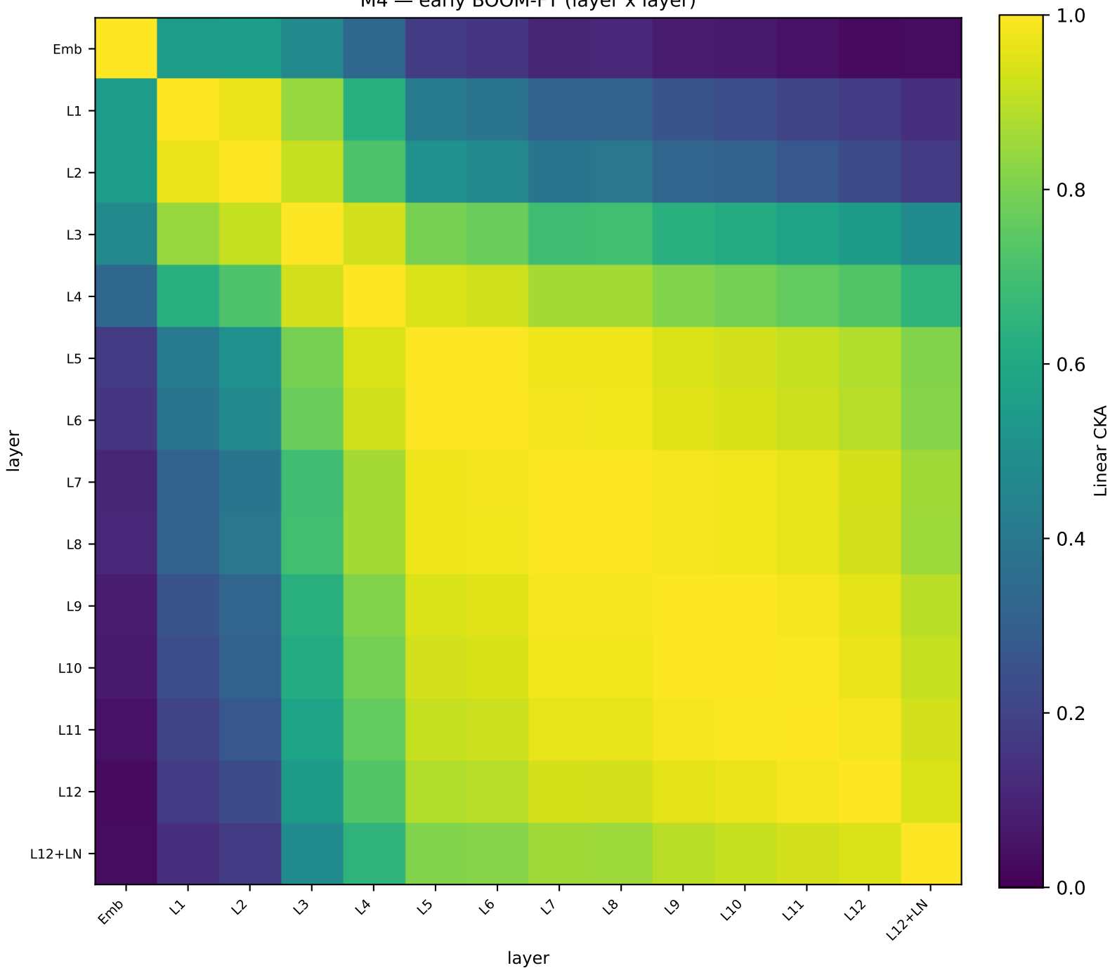
M4 — early BOOM-FT (layer x layer)
