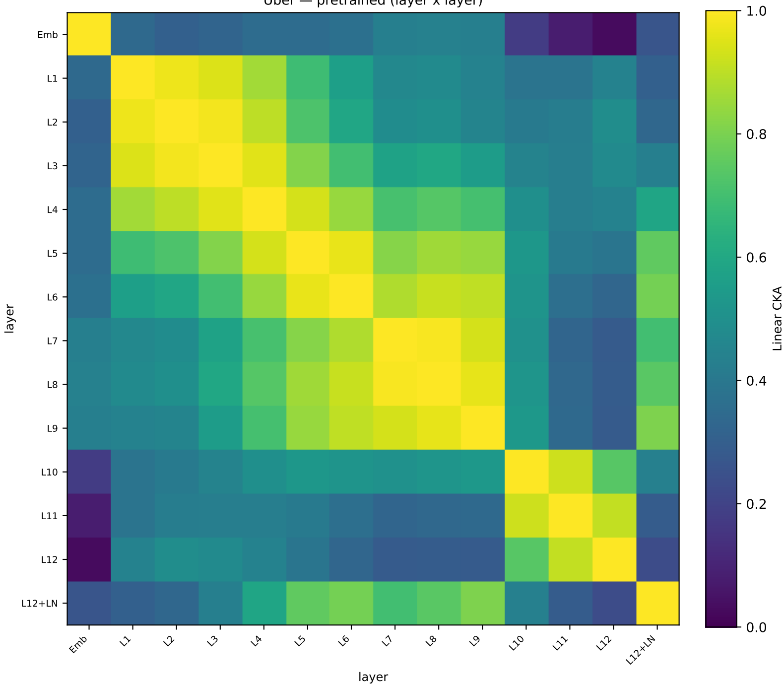
Uber — pretrained (layer x layer)
