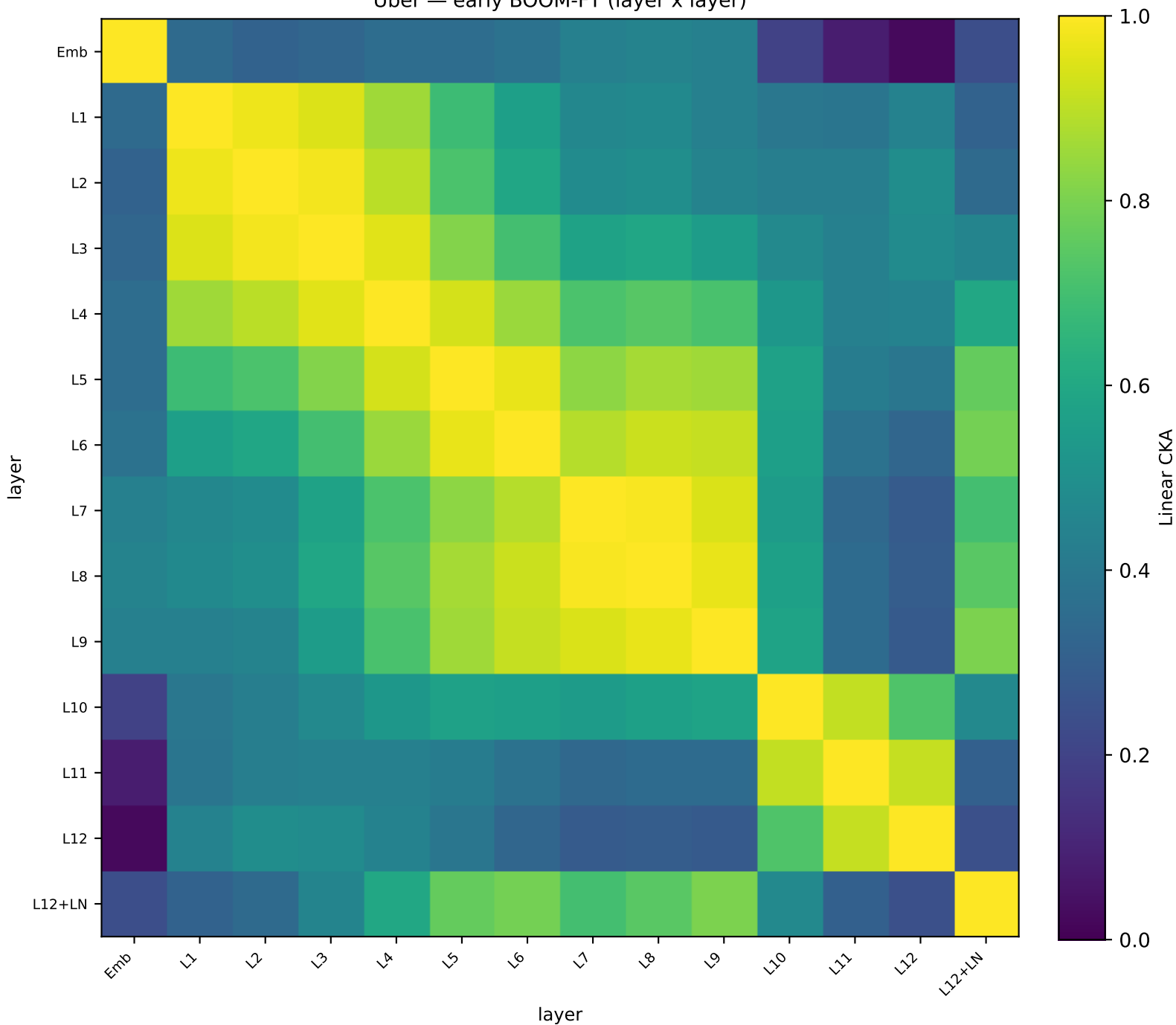
Uber — early BOOM-FT (layer x layer)
