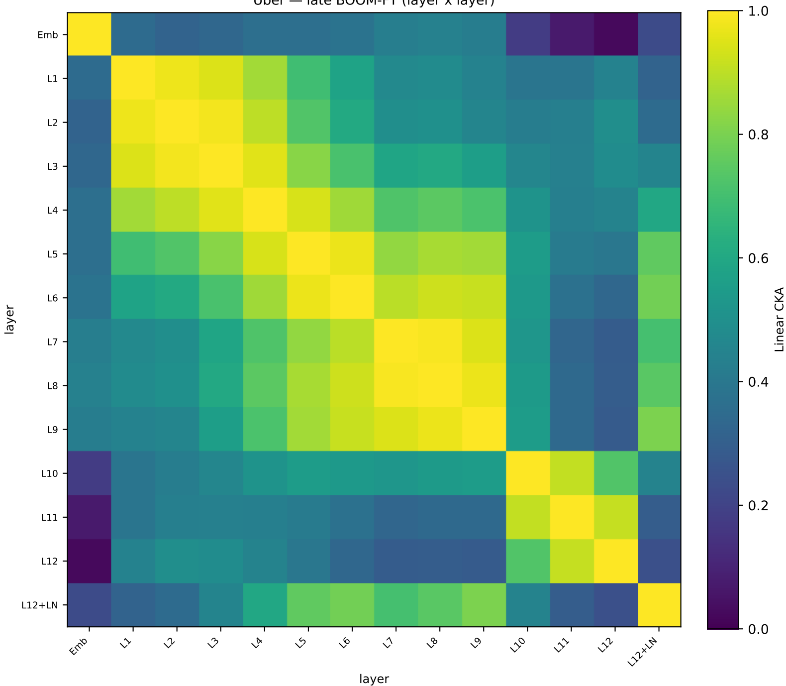
Uber — late BOOM-FT (layer x layer)
