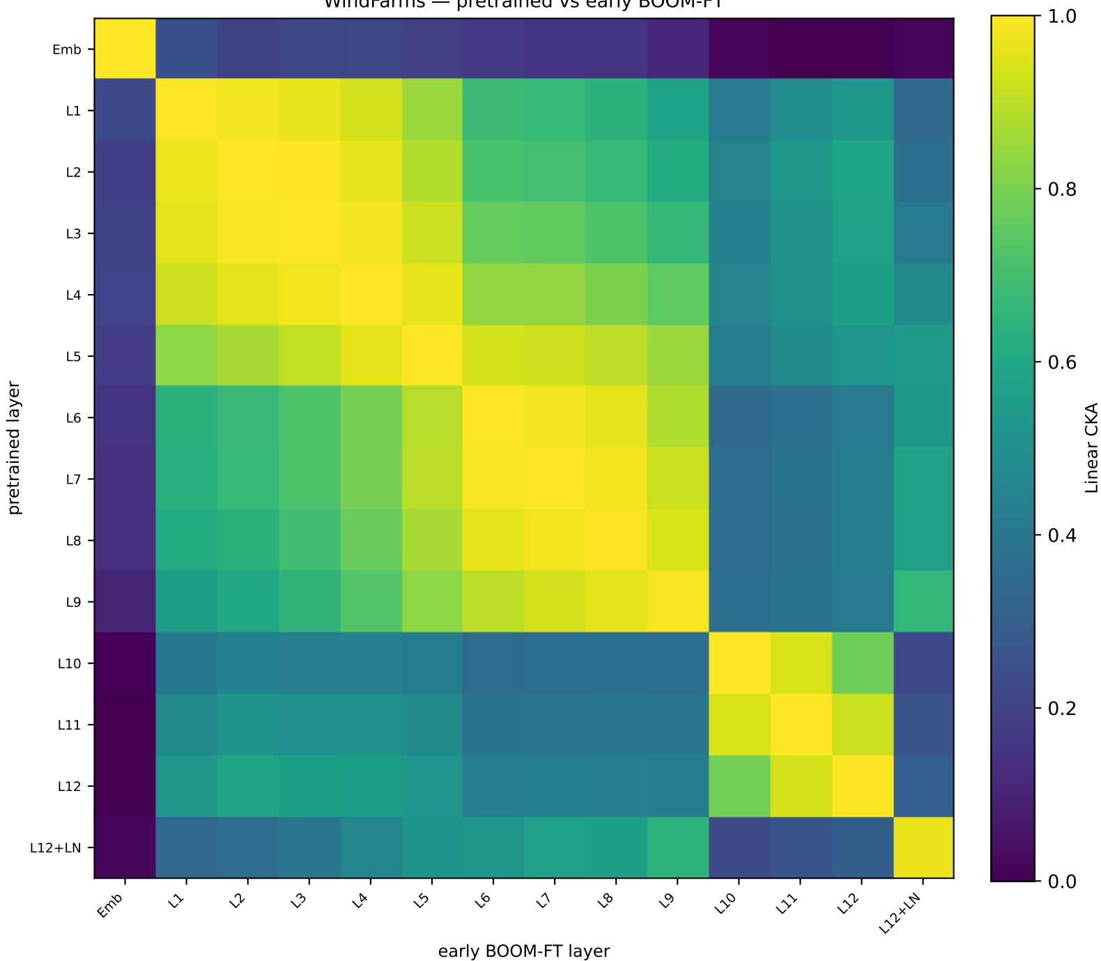
WindFarms — pretrained vs early BOOM-FT
