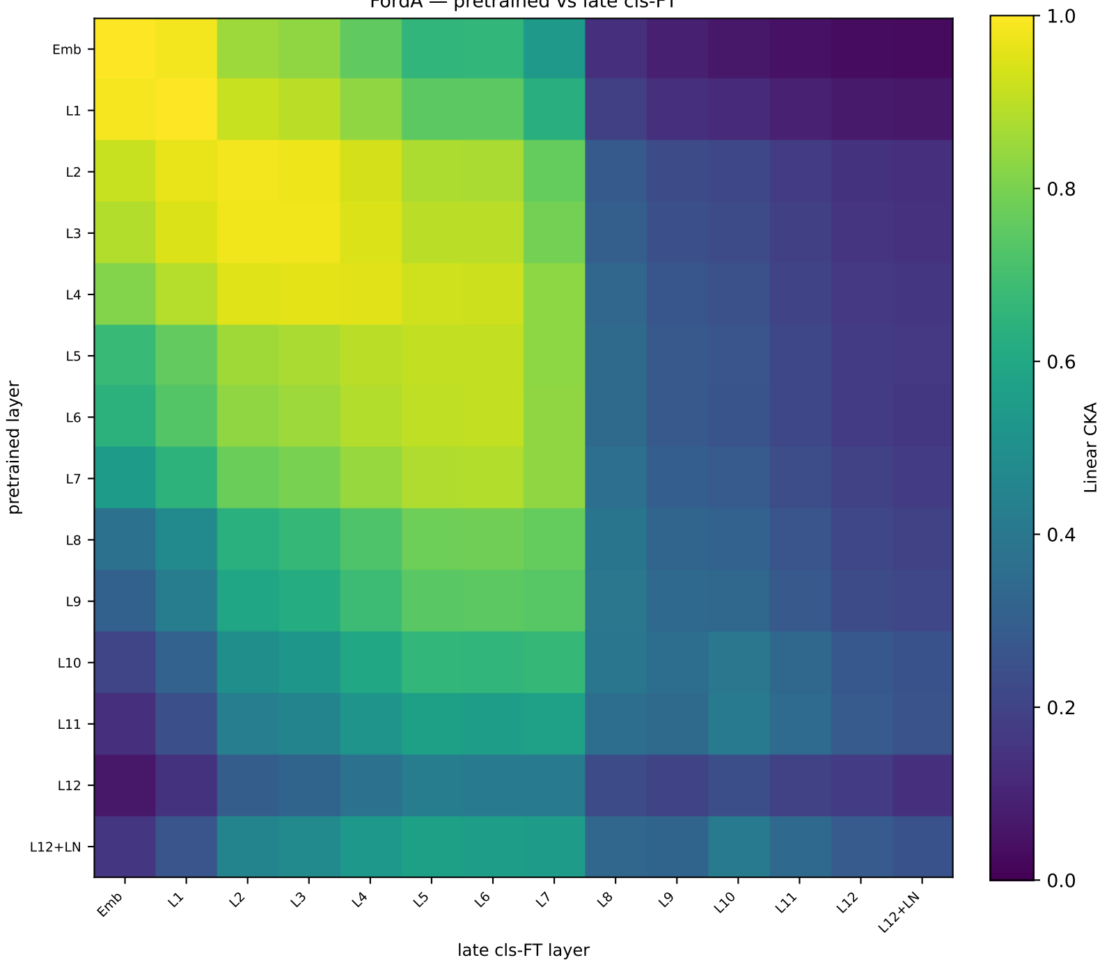
FordA — pretrained vs late cls-FT
