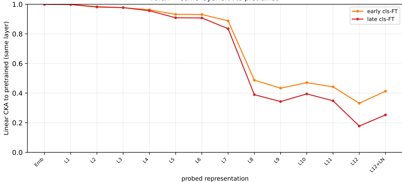
FordA — same-layer CKA to pretrained
