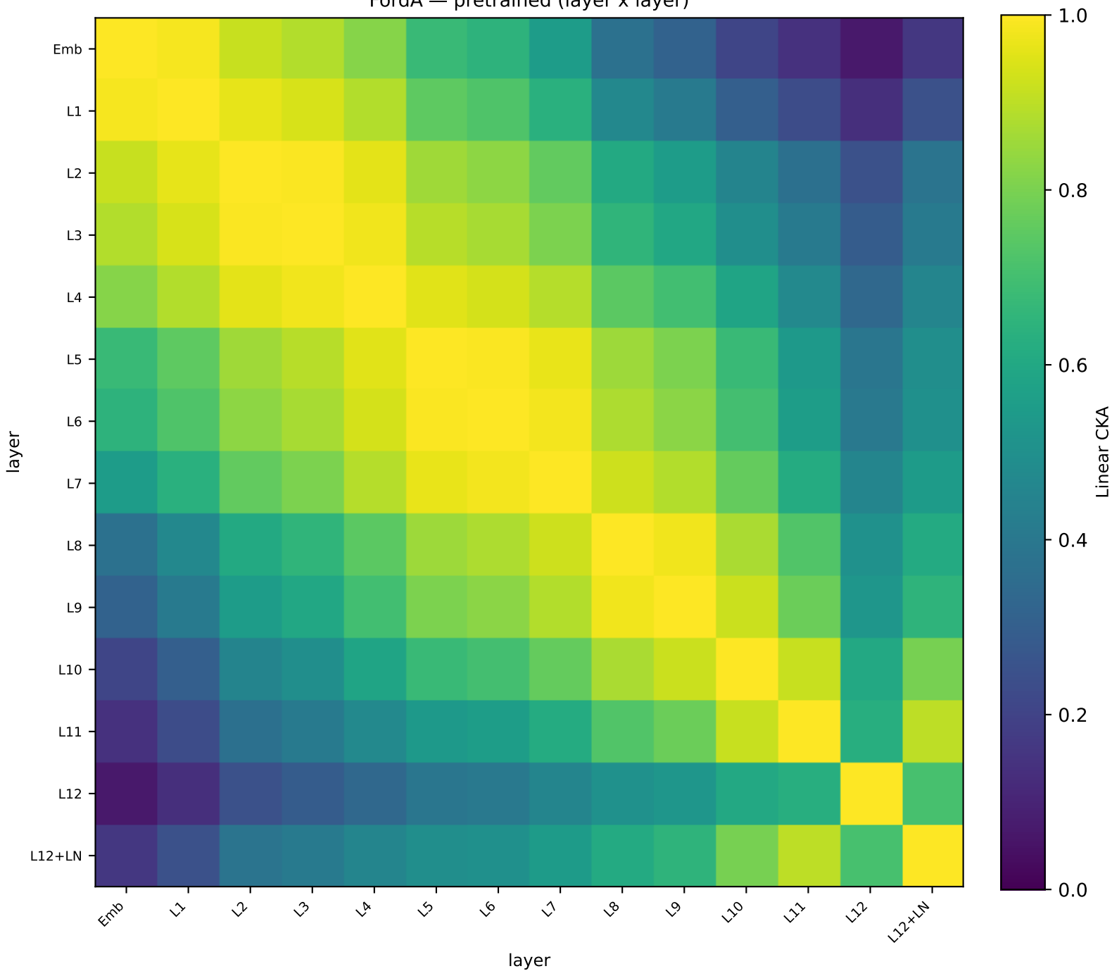
FordA — pretrained (layer x layer)
