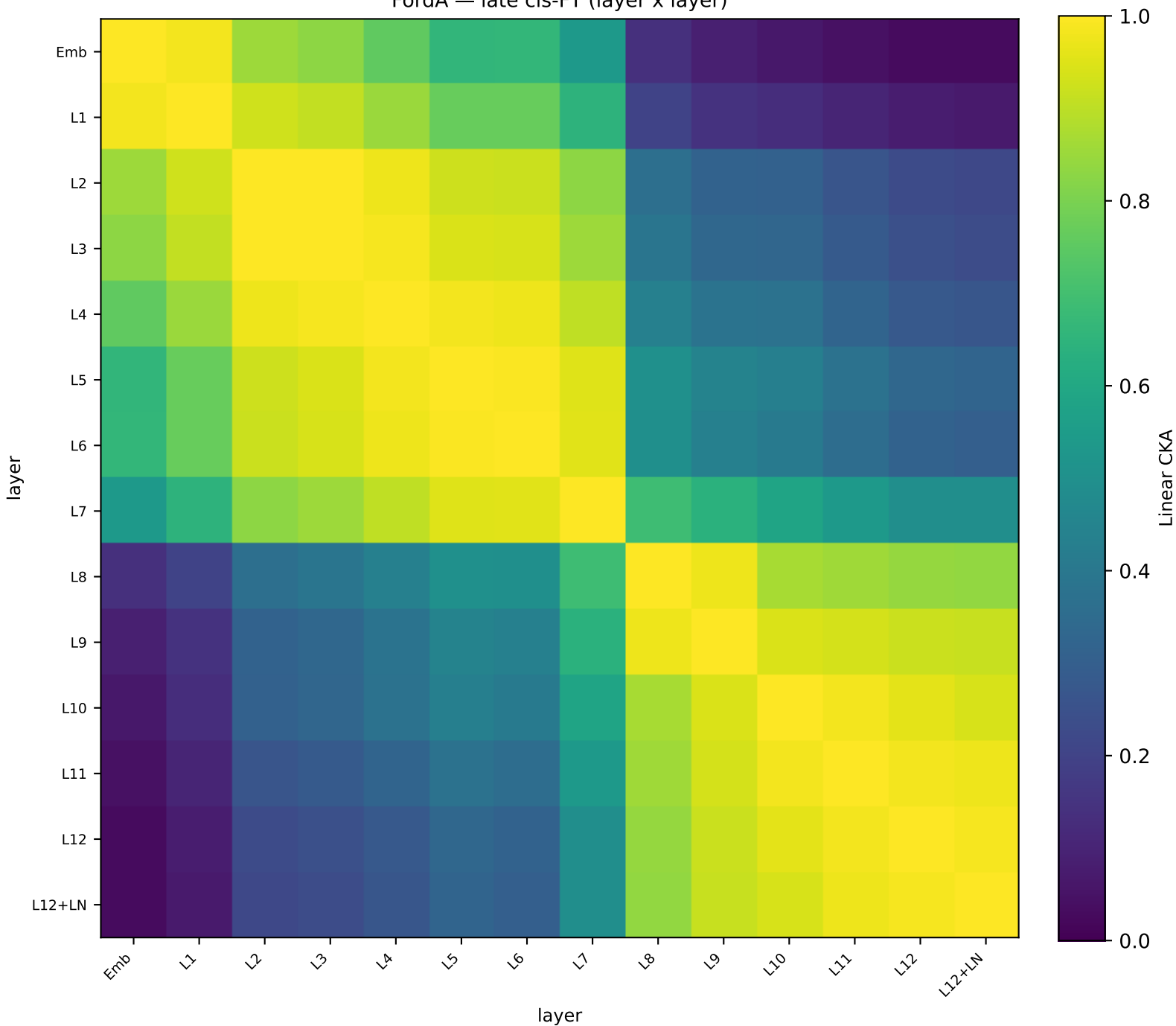
FordA — late cls-FT (layer x layer)
