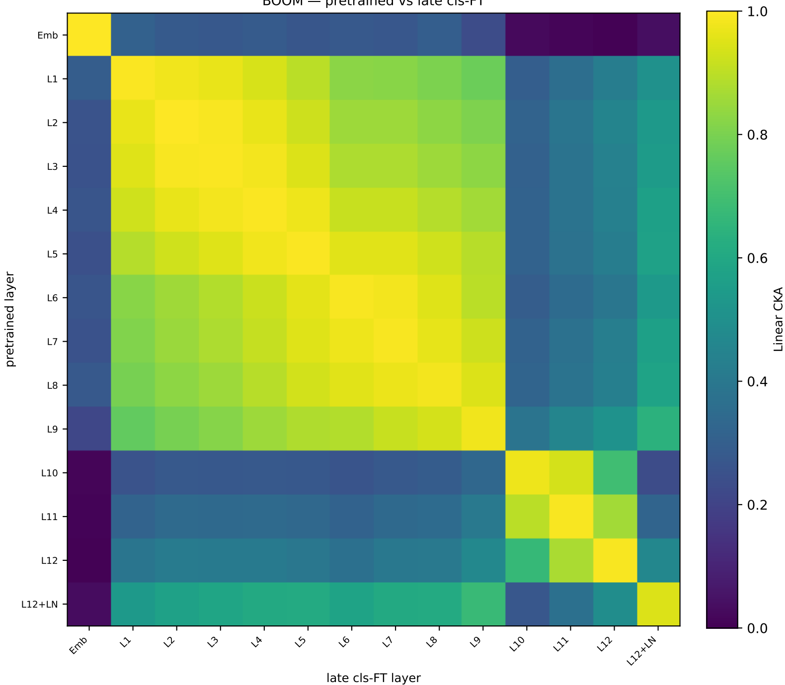
BOOM — pretrained vs late cls-FT
