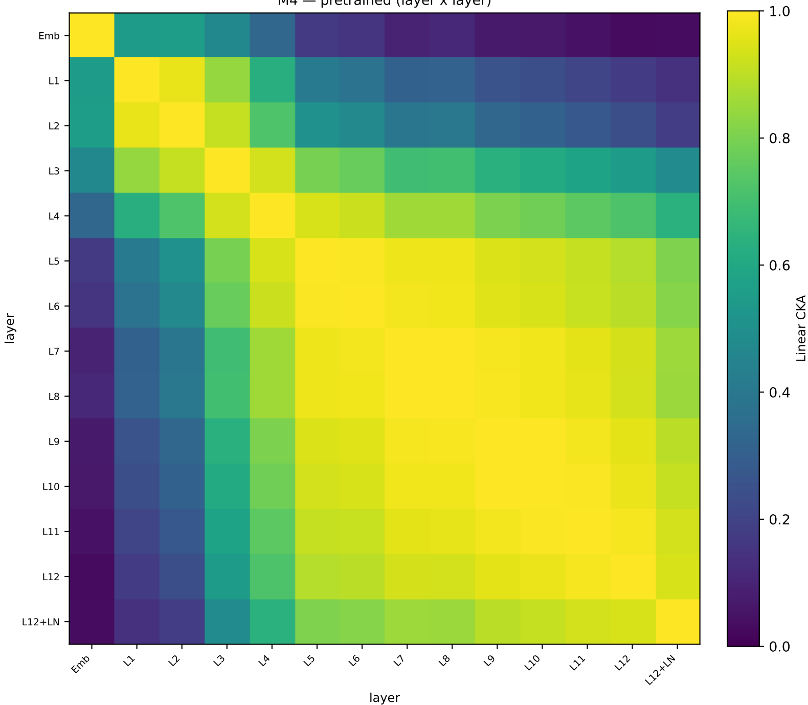
M4 — pretrained (layer x layer)
