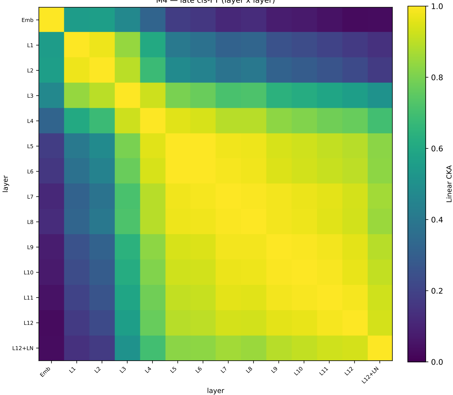
M4 — late cls-FT (layer x layer)
