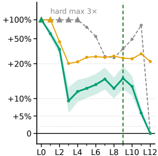
Electricity: test MASE increase over full model
