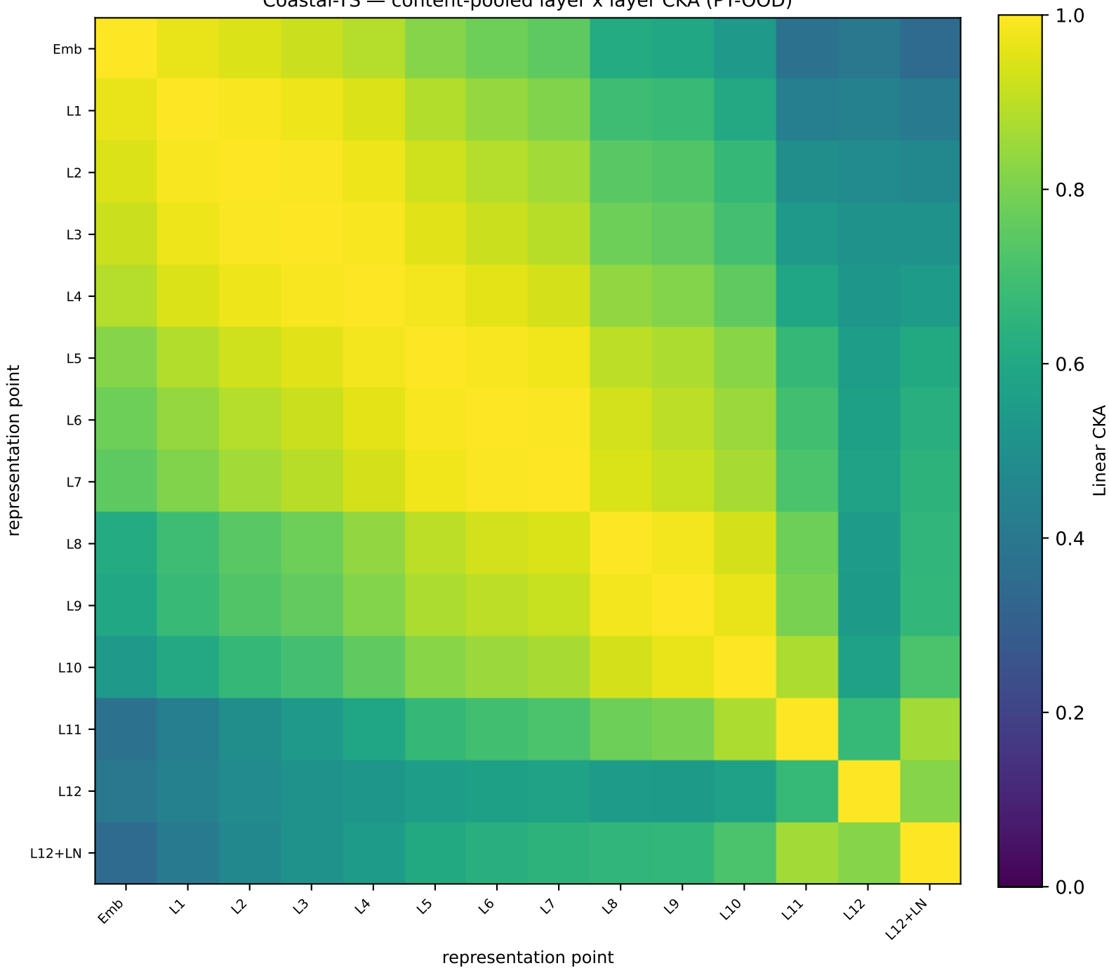
Coastal-TS — content-pooled layer x layer CKA (PT-OOD)
