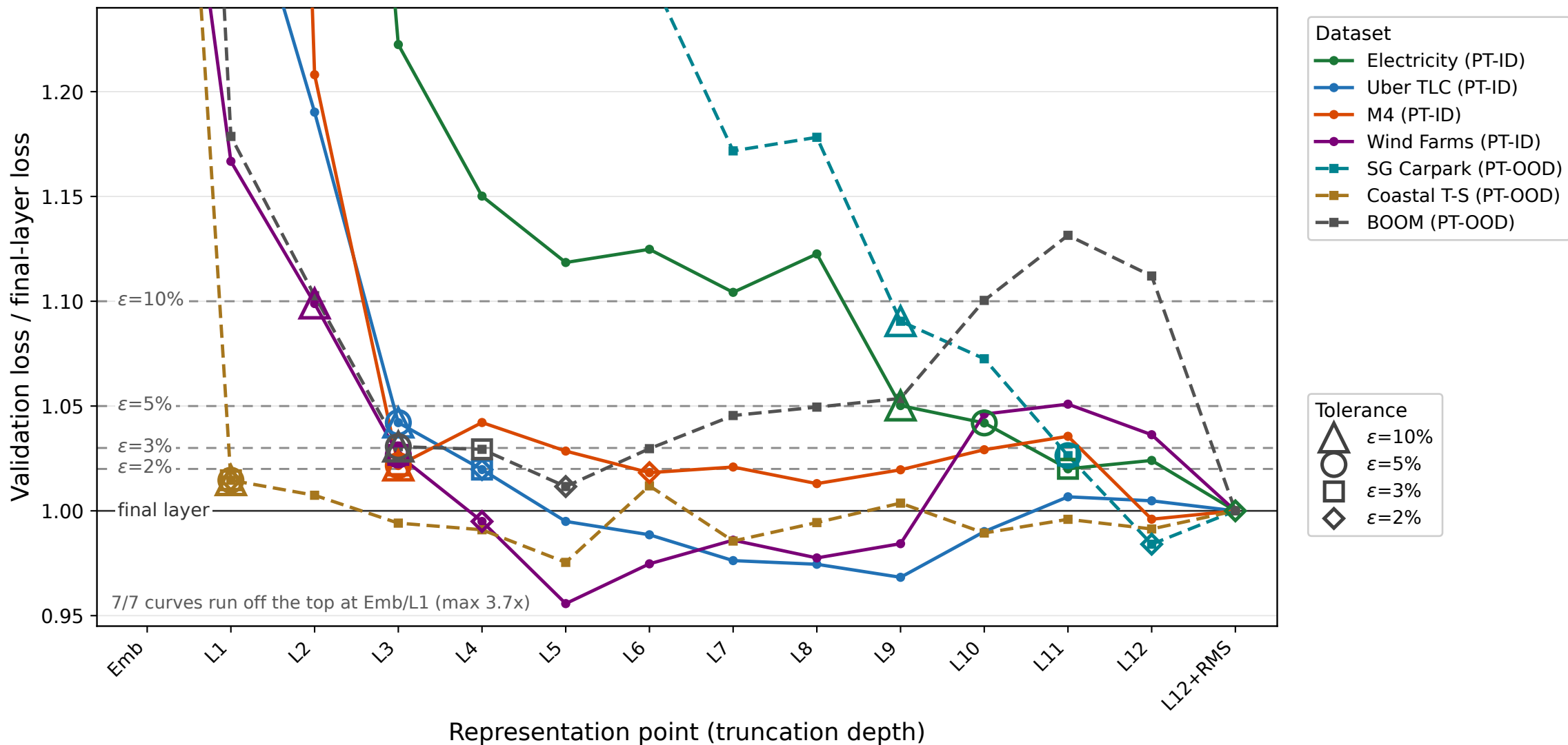
Where the saturation criterion cuts, as the tolerance \varepsilon varies open markers = the depth each \varepsilon selects
