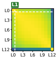
Coastal T-S
