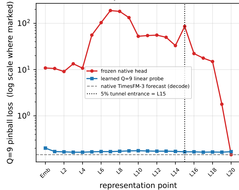
SG Carpark (PT-OOD, test N=354)
