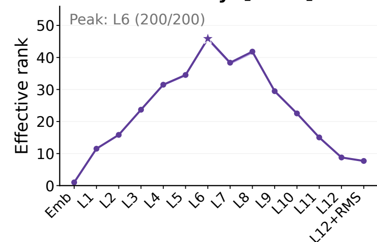
Electricity [PT-ID]
