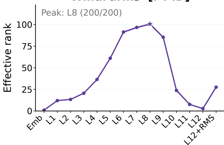
WindFarms [PT-ID]
