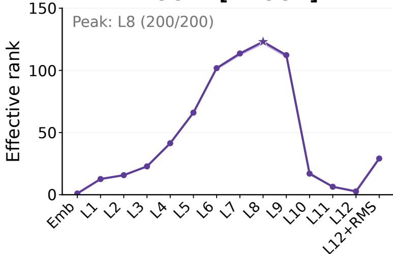
BOOM [PT-OOD]
