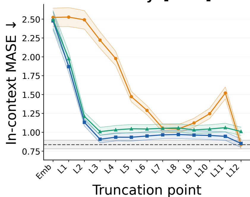
Electricity [PT-ID]
