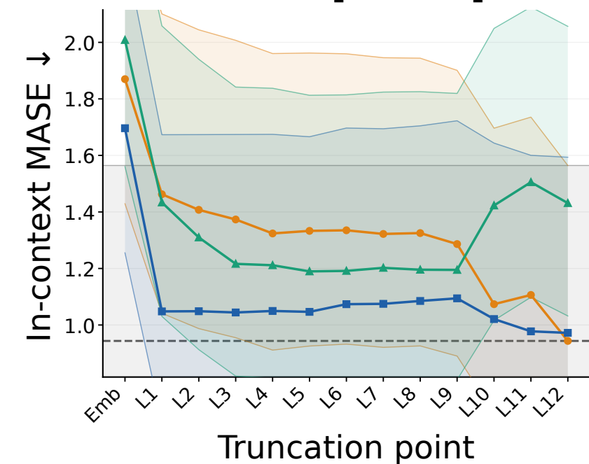
BOOM [PT-OOD]
