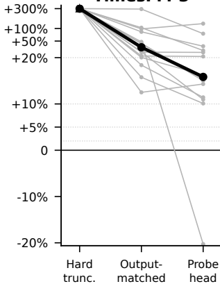
TimesFM-3
