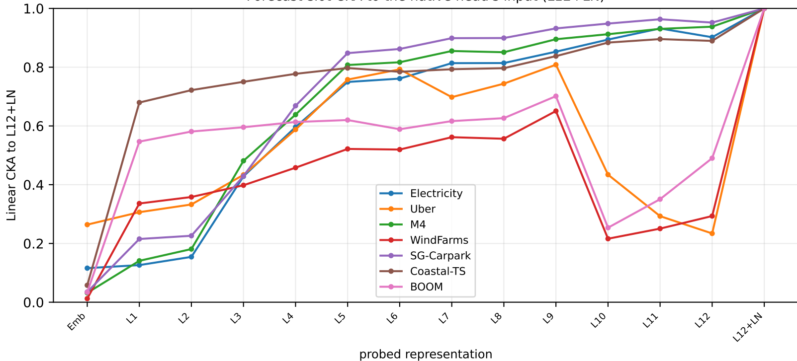
Forecast-slot CKA to the native head's input (L12+LN)
