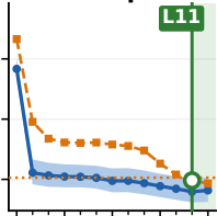
SG Carpark
