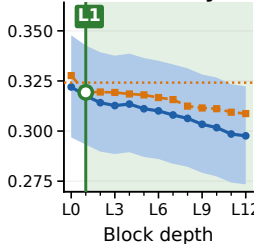
Wiki Daily
