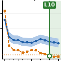
Electricity 15min
