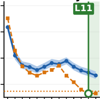
Electricity
