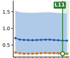
Wind Farms
