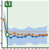
Coastal T-S
