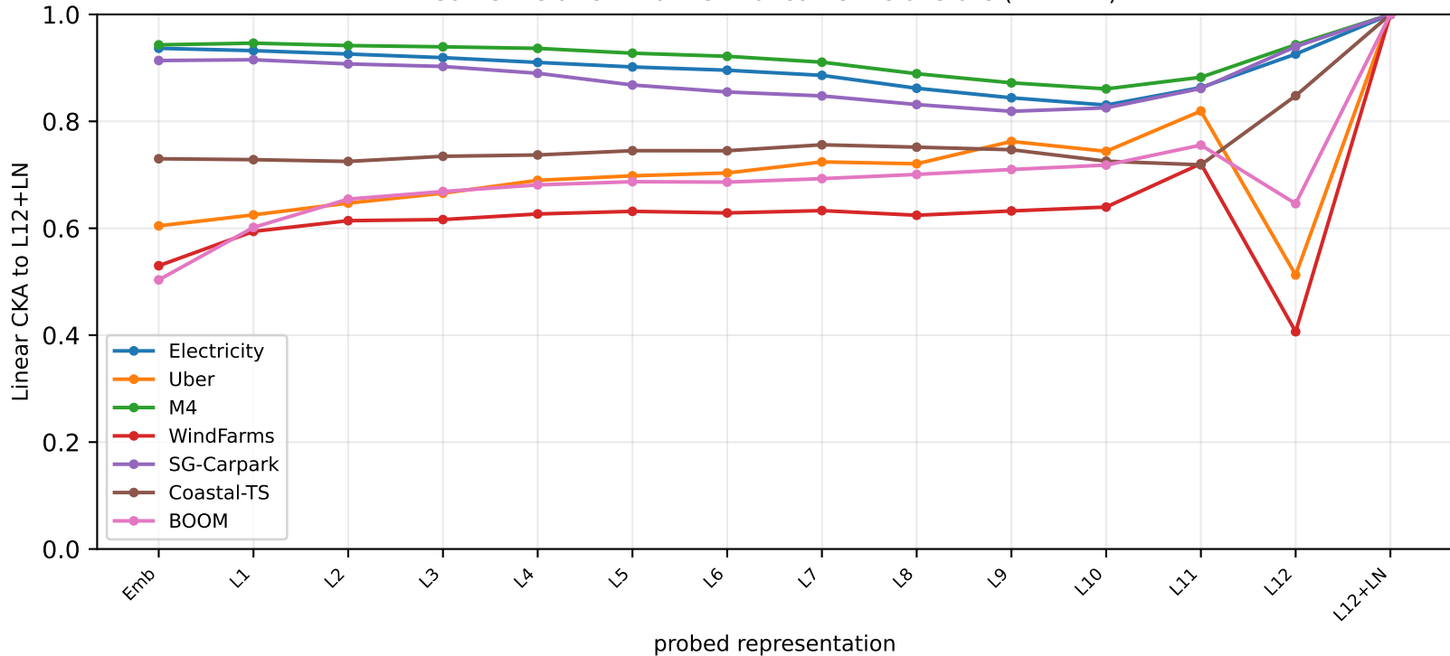
Content-slot CKA to the final content-slot state (L12+LN)
