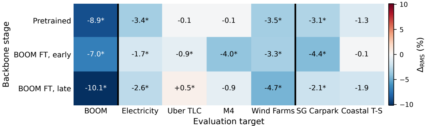
Effect of the final RMSNorm across BOOM fine-tuning stages
