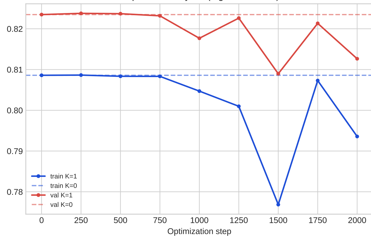
Depth boundary F1 (higher is better)
