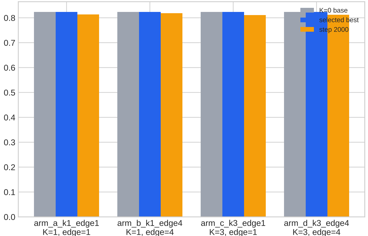
Validation depth-boundary F1 (higher is better)
