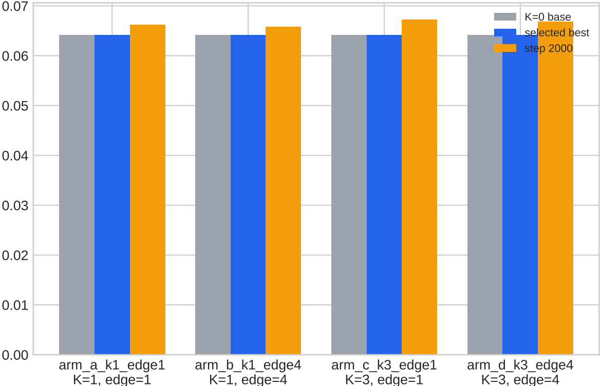
Validation aligned point Rel (lower is better)
