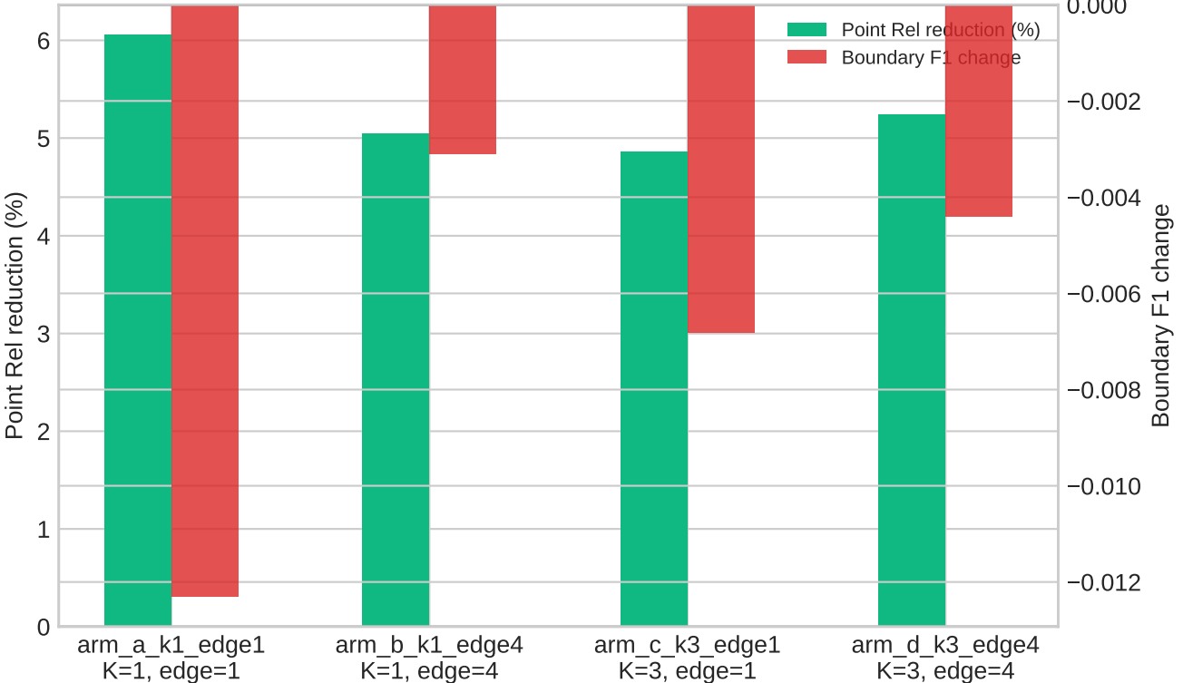
Latest checkpoint: training split
