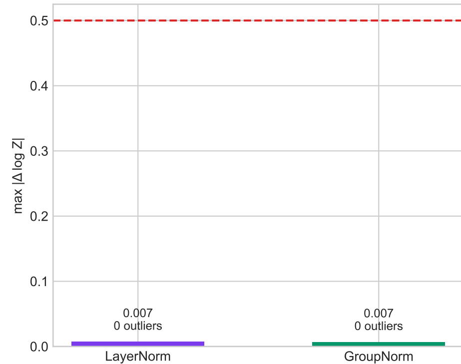
Residual safety over 132 images
