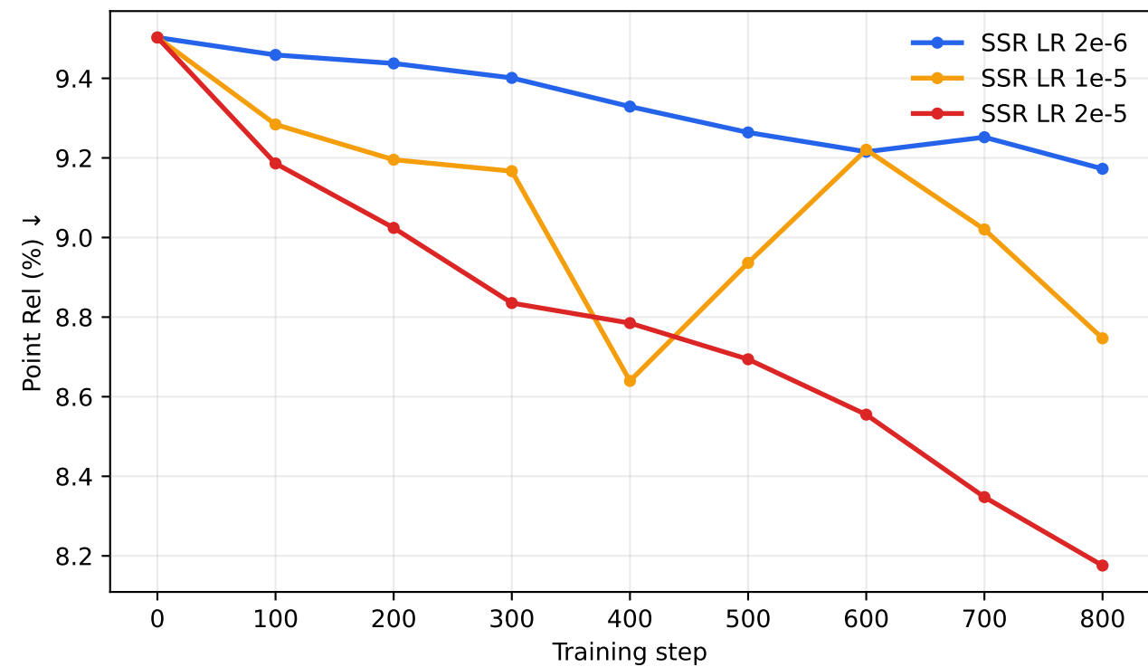
Validation locked-structure Point Rel
