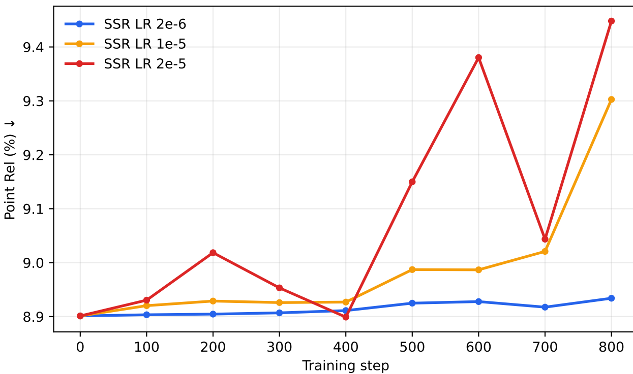
Validation full Point Rel
