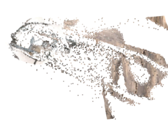
K=1 novel view proposal point Rel 7.02%
