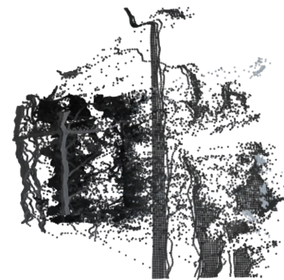
K=3 novel view proposal point Rel 11.32%
