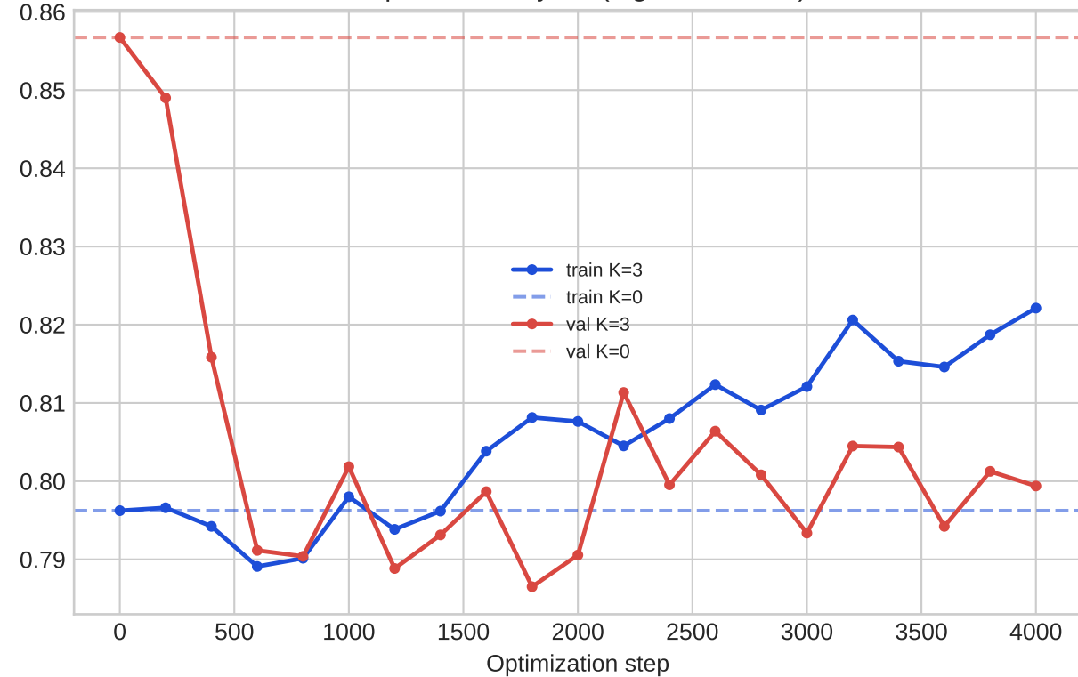
Depth boundary F1 (higher is better)
