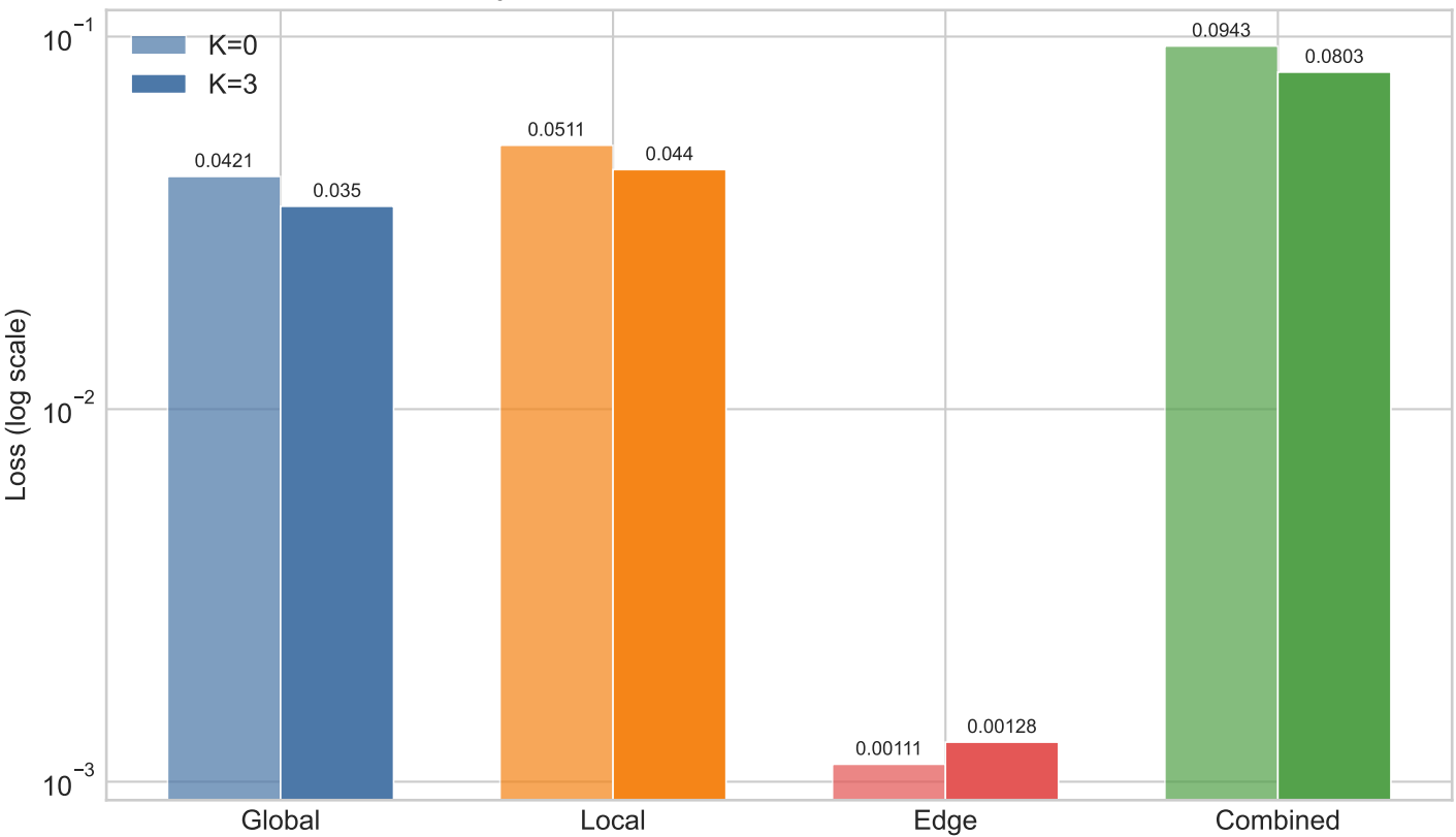
Objective scalar values on locked train ROIs
