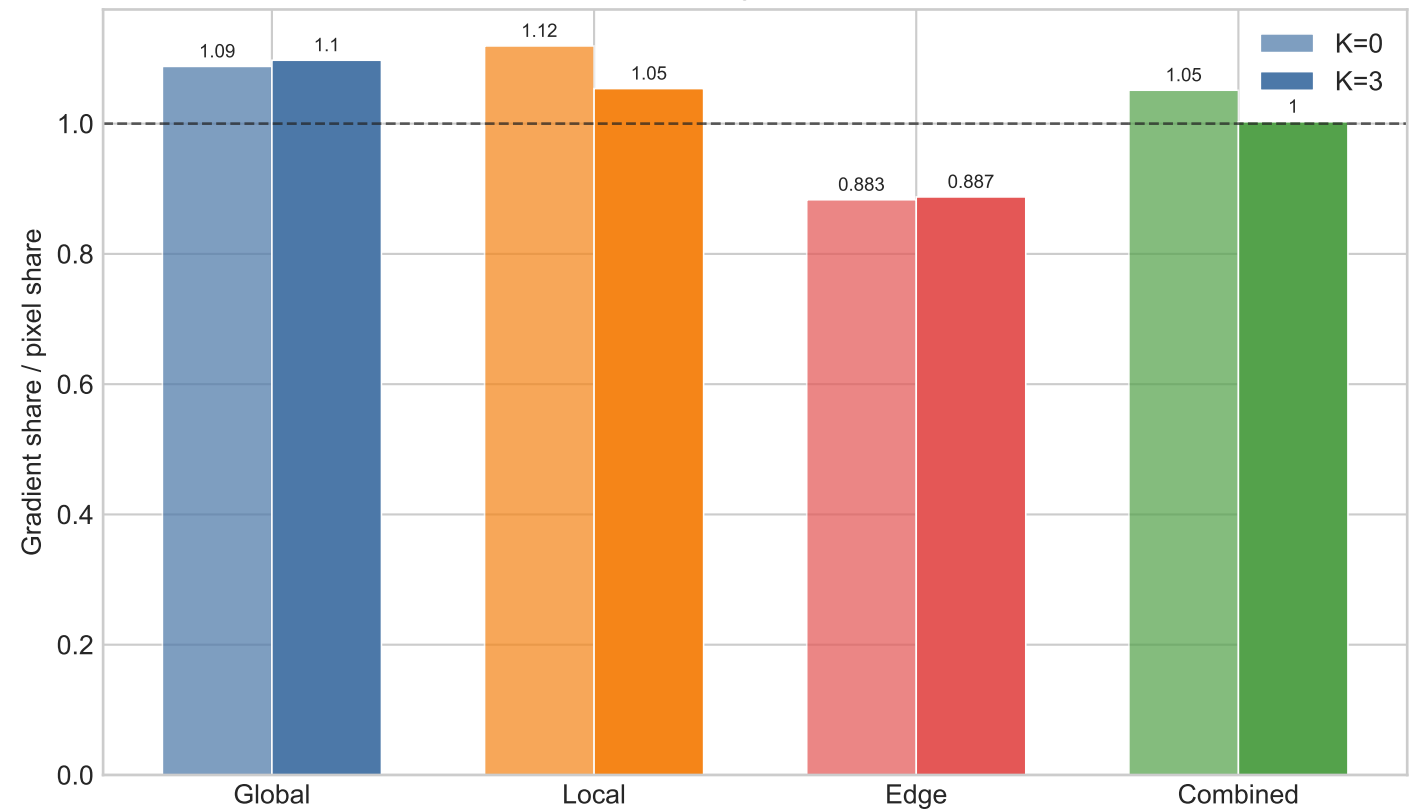
Locked structure gradient enrichment
