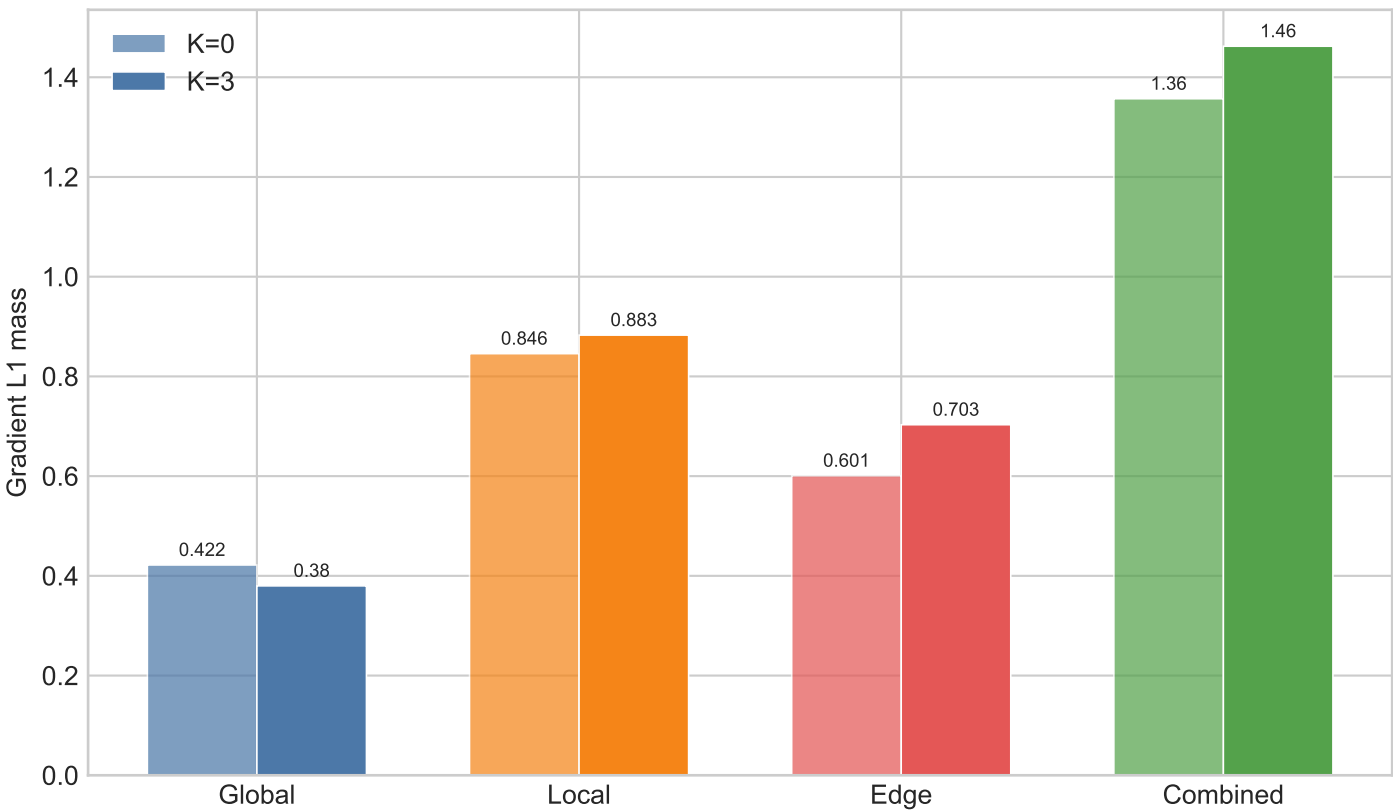
Direct objective pressure on per-pixel \zeta = \log Z
