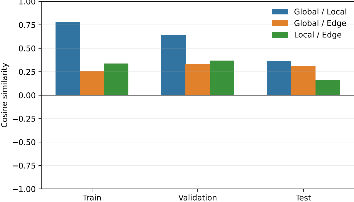
Alignment inside 3D U-Net (output layer excluded)
