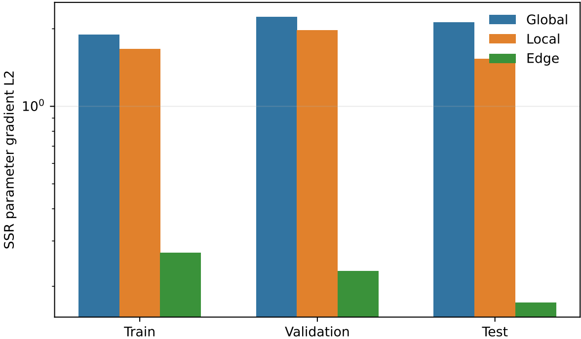
Gradient strength after SSR Jacobian
