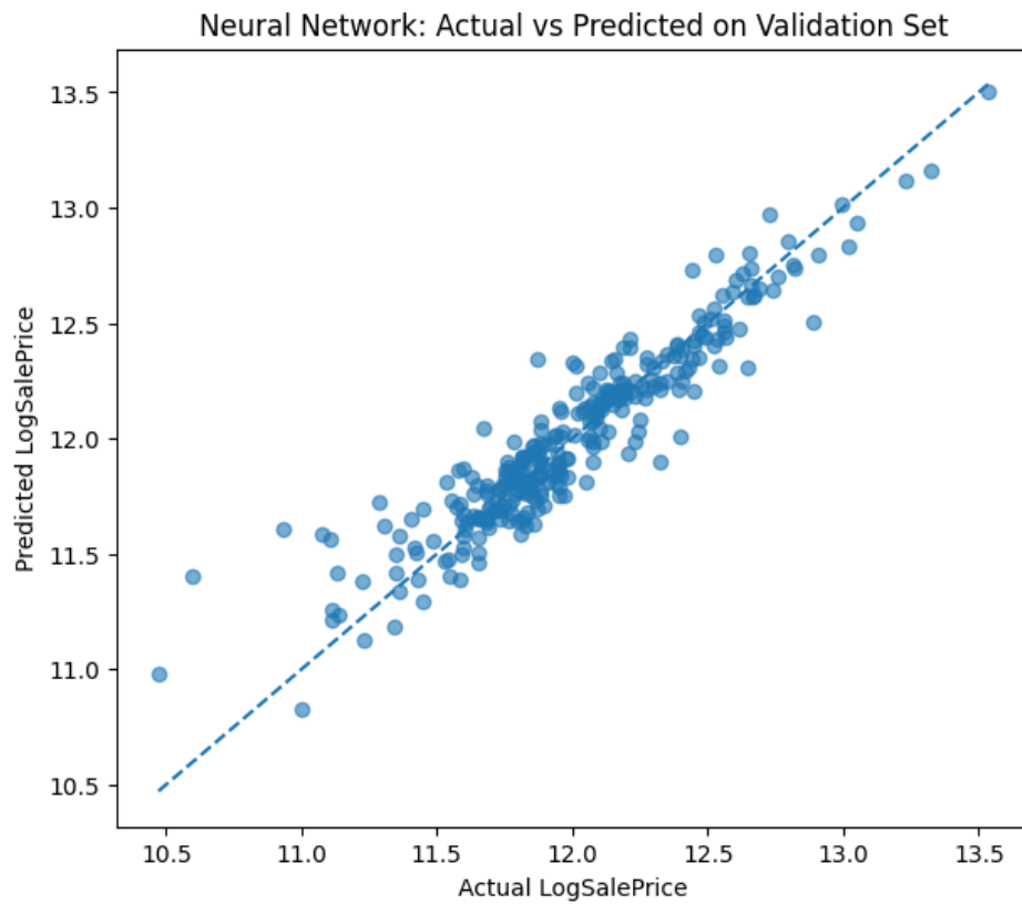
Figure 8: Actual versus predicted LogSalePrice values on the validation set for the selected neural network.
