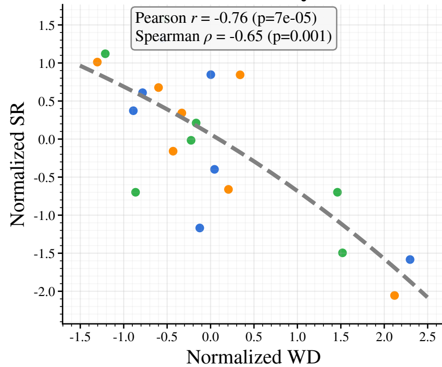
Visual-only
