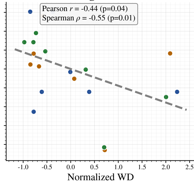
Target-Real
