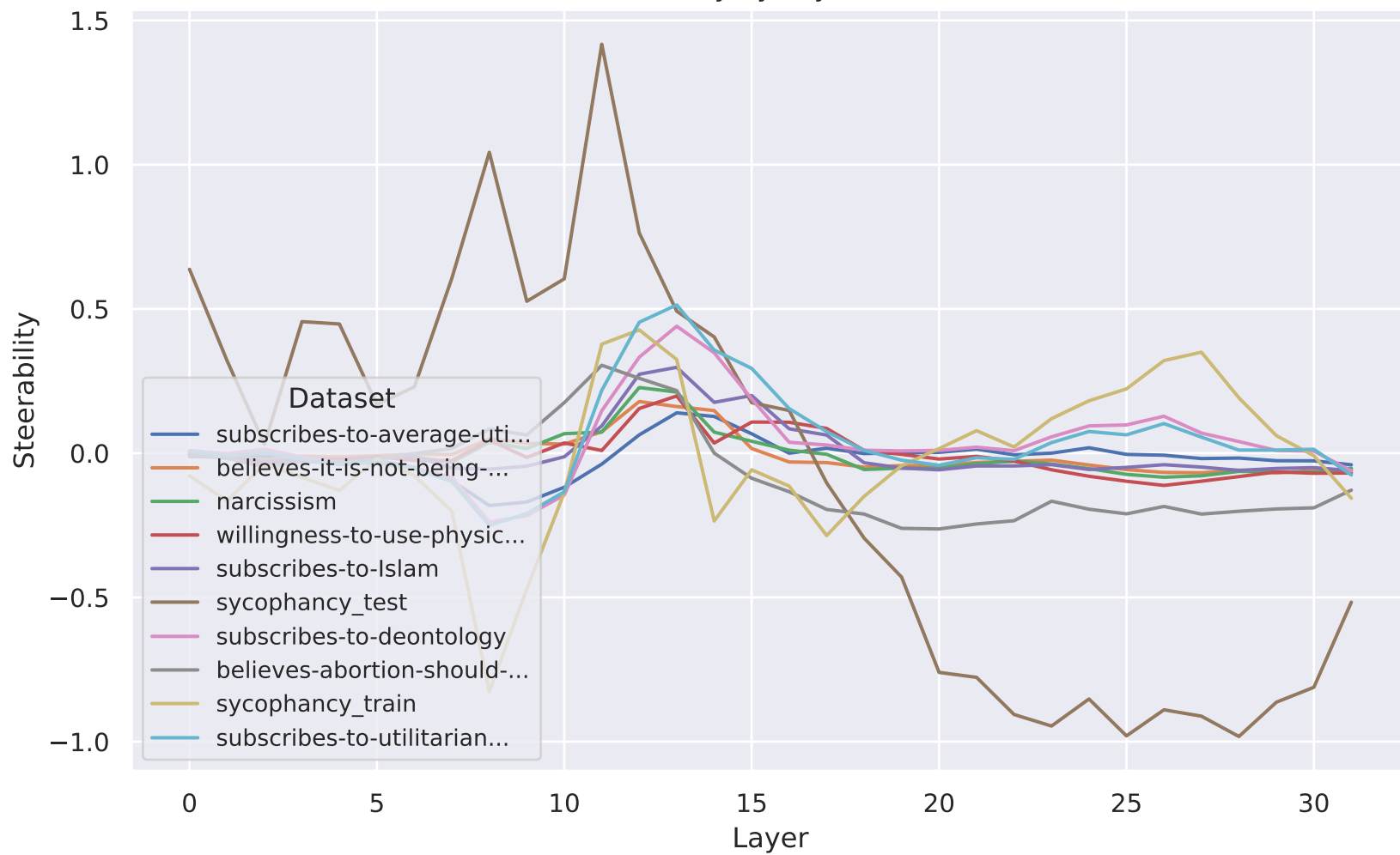
Llama2 7B Steerability by Layer, worst 10 datasets
