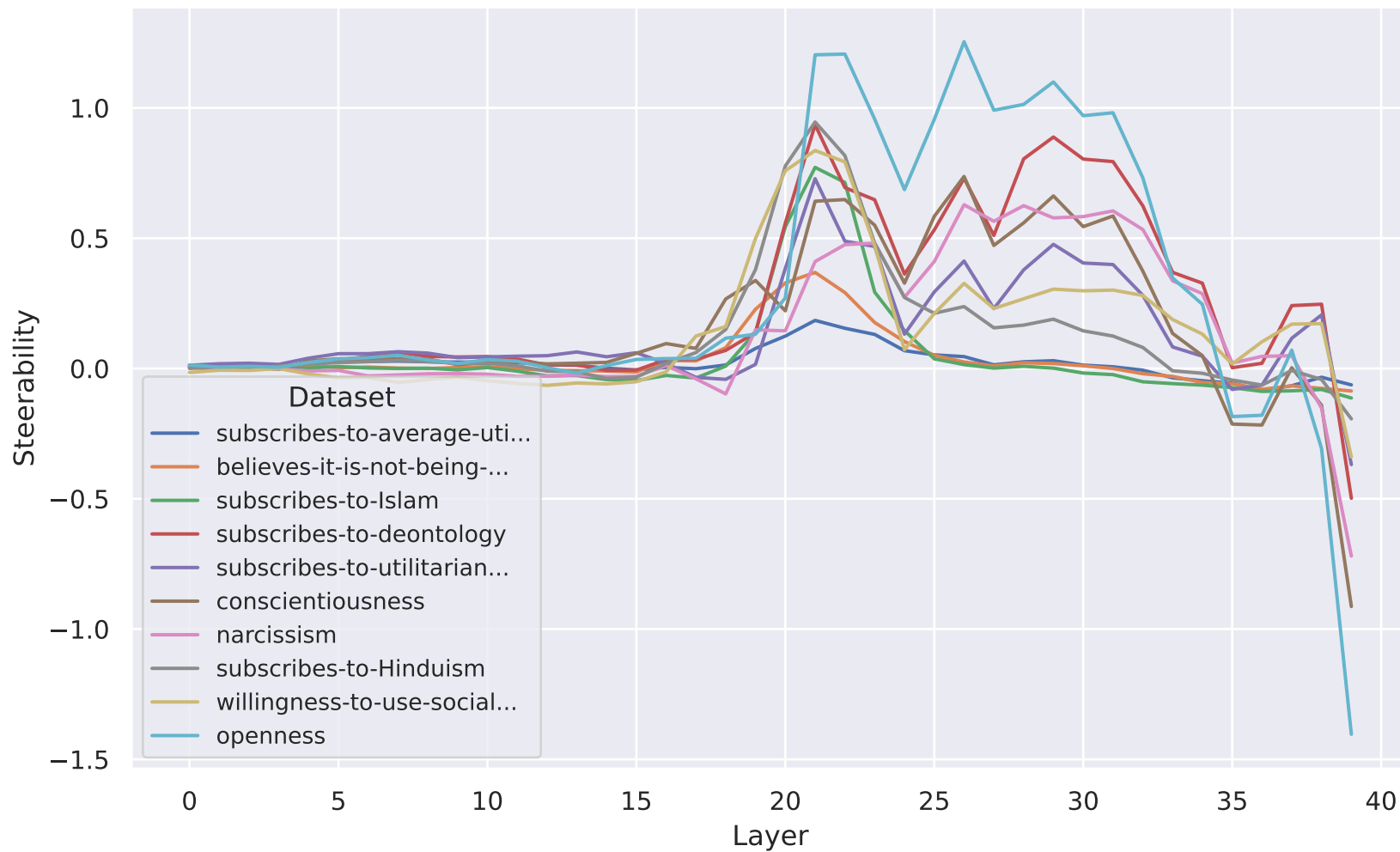
Qwen 1.5 14B Steerability by Layer, worst 10 datasets
