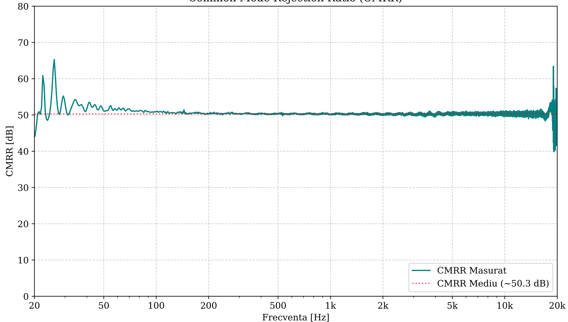
Common Mode Rejection Ratio (CMRR)
