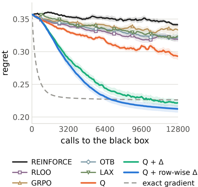
Regret for DFL Black-box
