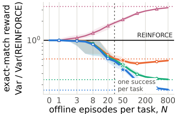
variance at the warm start
