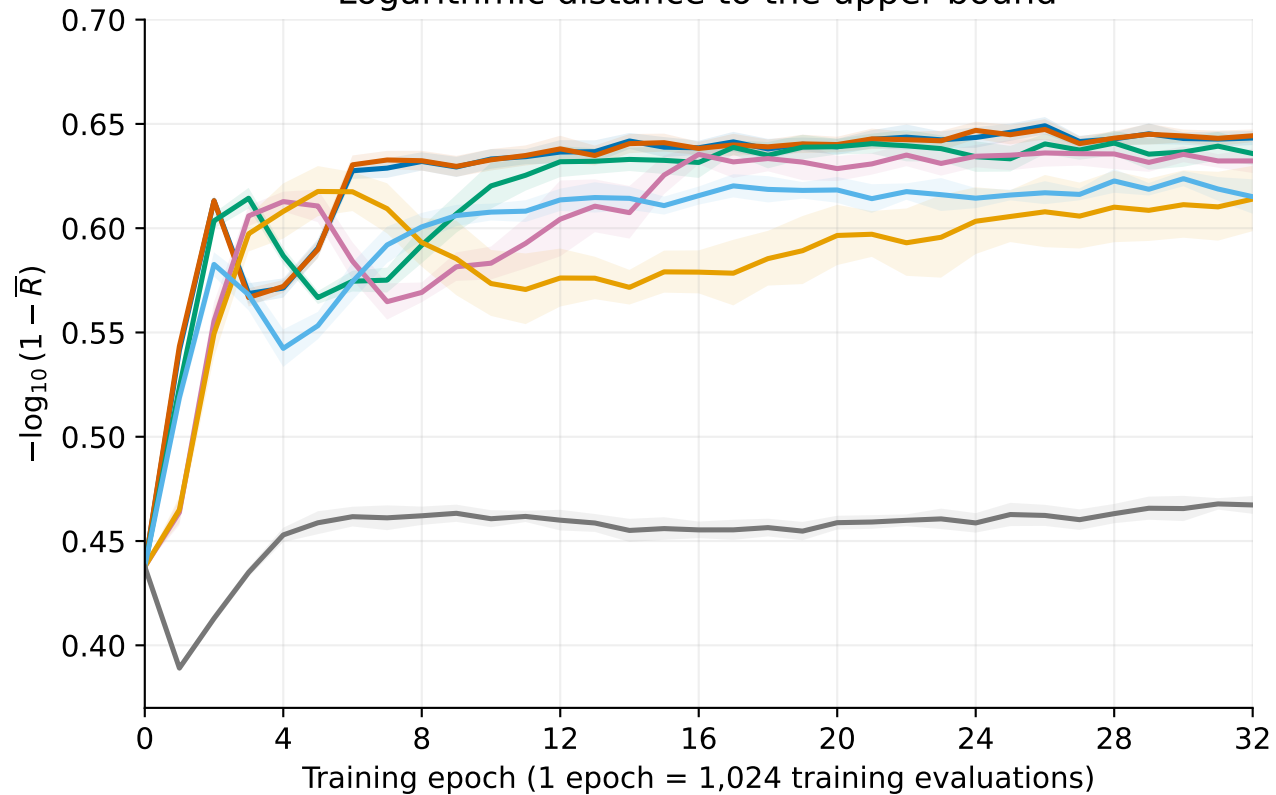
Logarithmic distance to the upper bound
